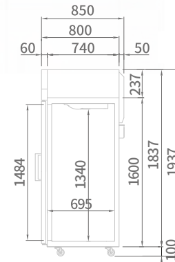
SIDE VIEW (Glass Door)
