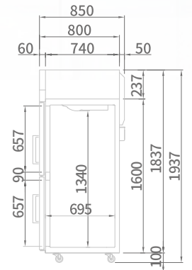
SIDE VIEW (Half Glass Door)
