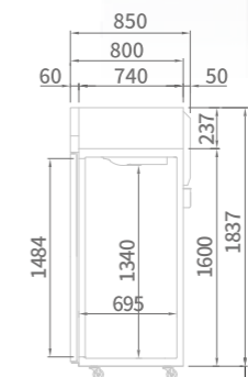
SIDE VIEW (Full Door)
