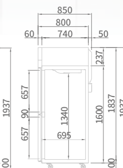
SIDE VIEW (Half Door)
